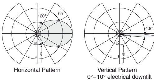
1920 – 2200 MHz: +45°/–45° Polarization
