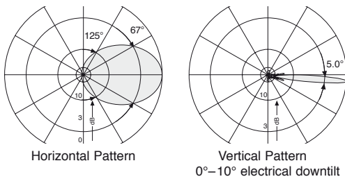
1850 – 1990 MHz: +45°/–45° Polarization
