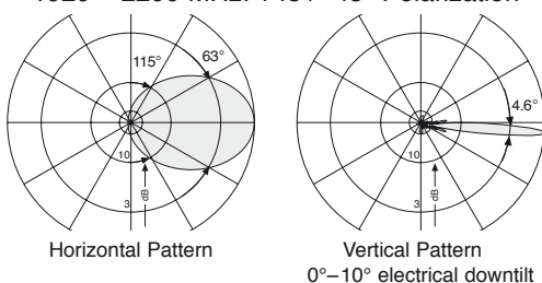
1920 – 2200 MHz: +45°/–45° Polarization
